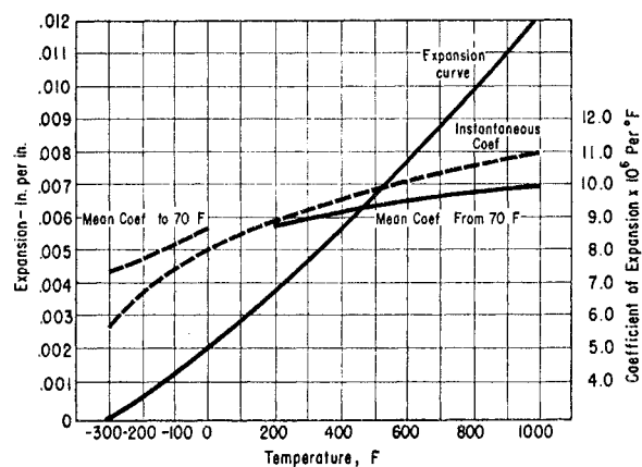
Fig. 5. Thermal expansion of Type 304 stainless steel from -300 F to 1000 F.
